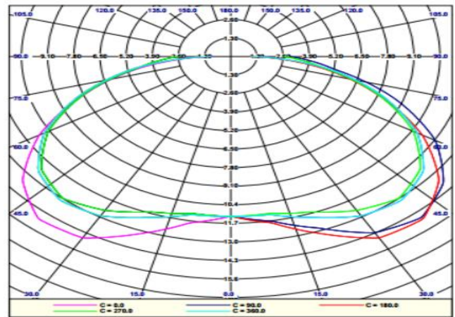
Luminous Intensity Distribution
